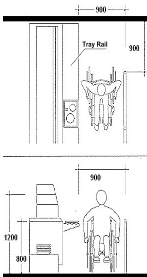
Figure E7-2: Wheel chair, aisle and reach height
