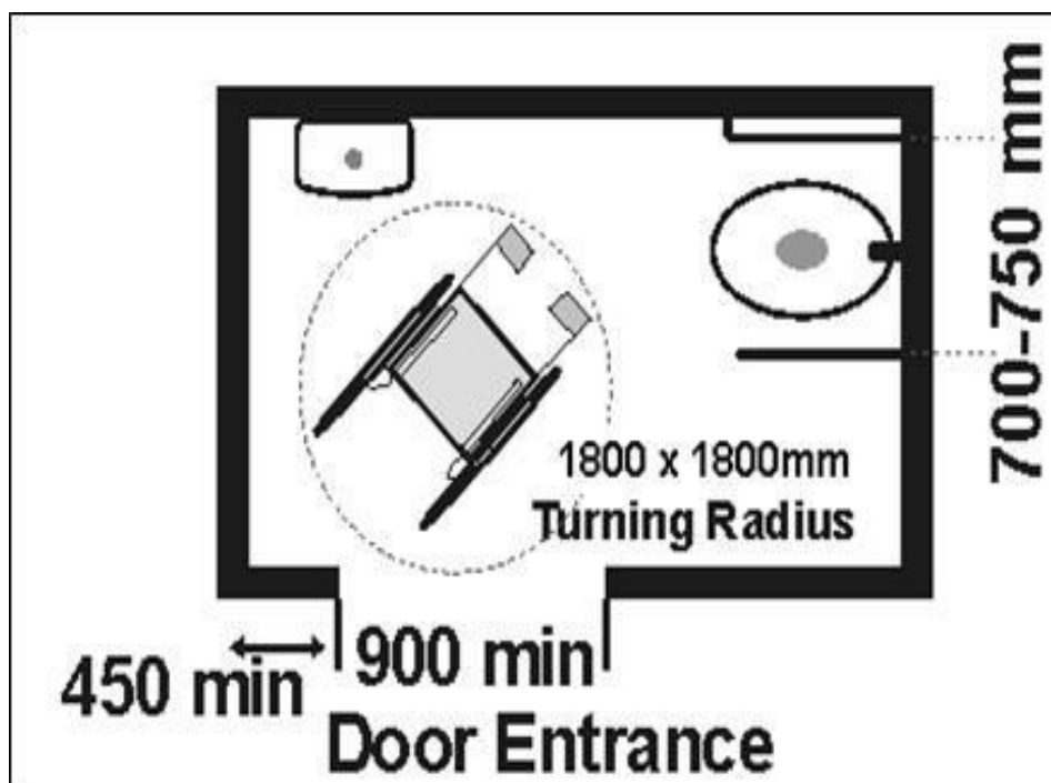
Figure E6-1: Wheelchair maneuvering space in toilet
